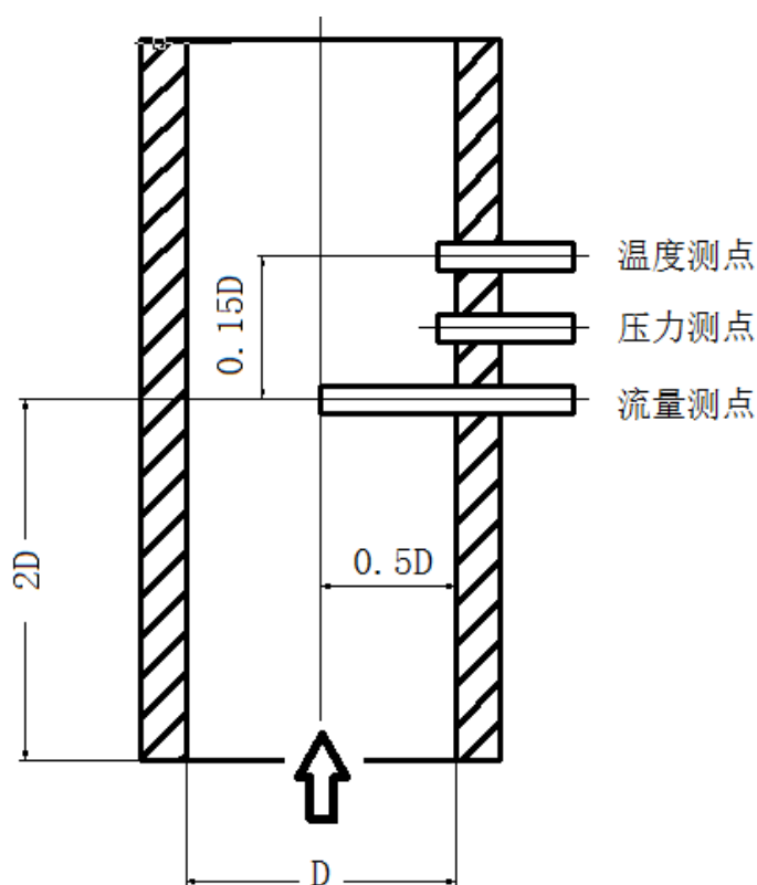
图3 烟气管道测点布置
